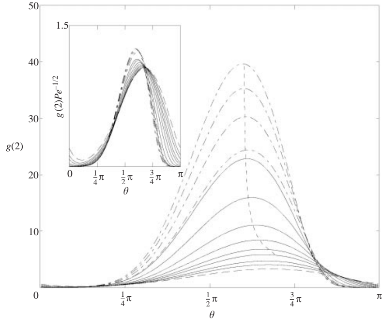
FIGURE 10. The non-equilibrium pair-distribution function at contact in the shear flow-gradient plane as a function of \theta and Pe for hard spheres with hydrodynamics ( b/a = 1.00001 ). Results from the solution of the full Smoluchowski equation are shown as solid lines and the solutions from the boundary-layer equation are shown as dashed curves. From bottom-to-top: Pe = 10 (dashed line), 15, 20, 30, 40, 60, 100, 200 and 400 (bold line); and from the boundary-layer equation Pe = 400 , 600, 800 and 1000. The short-dashed curve is a best fit to the maxima in g(2) . The inset shows that scaling by Pe^{1/2} reduces the maximum in the compressional quadrant to O(1) .
