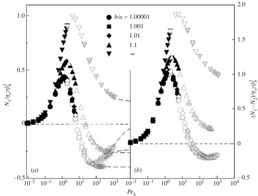
FIGURE 19. (a) The first normal stress difference and (b) the difference between the first and second normal stress differences at O(\phi_b^2) as functions of Pe_b and excluded volume parameter b/a . Filled black symbols, surface spherical harmonic expansion; open symbols, finite-difference solution; tinted symbols, finite-difference solution of the boundary-layer equation; dashed lines, extrapolation of large Pe_b results.
